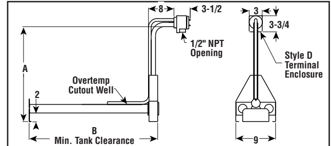
Dimensions (Inches)
